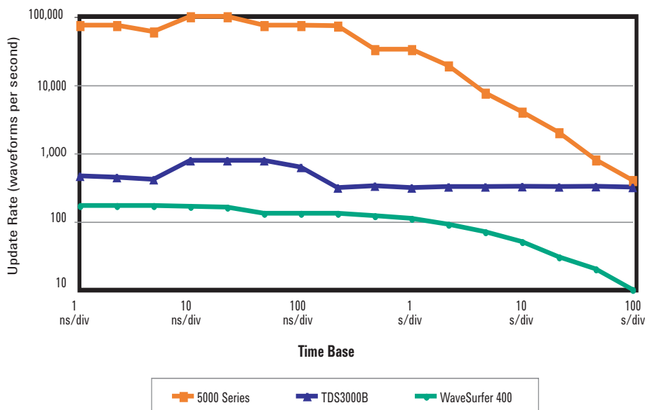
Figure 5. Update rates of popular oscilloscopes using their default real-time time acquisition mode
