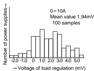
[Fig.-4] Distribution of Load Regulation (CV Characteristics)
